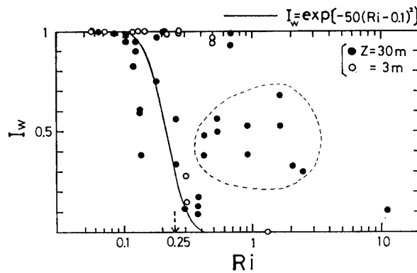
Fig. 4. Variation of intermittency factor I_w with Ri for stable condition. The solid line is from eq. (4) and the symbols are the same as those in Fig. 3.
