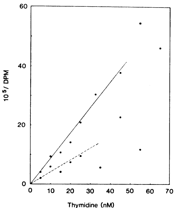
Fig. 5. Plots of reciprocal of [methyl- ^3\text{H} ] thymidine incorporation into TCA insoluble fraction. Closed circle: Stn. 2; open circle: Stn. 4.
