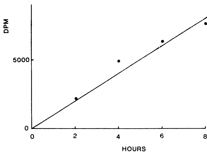
Fig. 2. Time course of [methyl- ^3\text{H} ] thymidine incorporation into TCA insoluble fraction.
