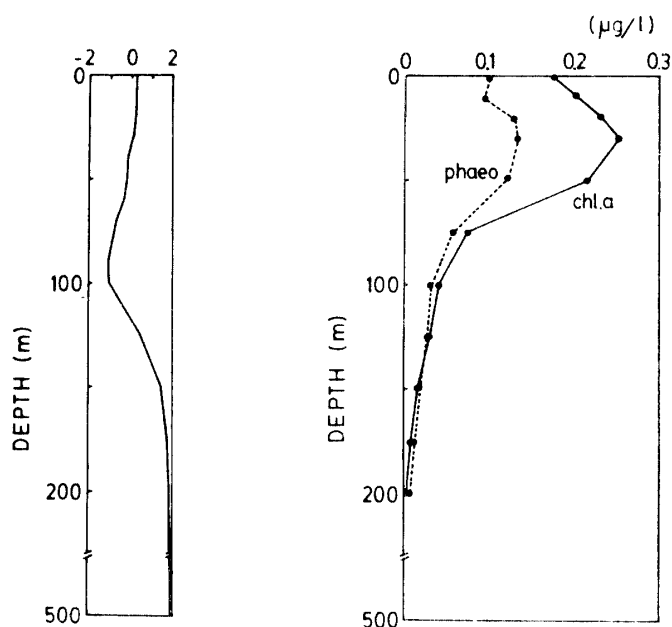
Fig. 3. Vertical profile of temperature and chlorophyll a at Stn. 3B (from the Preliminary Date Report).
