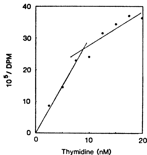
Fig. 6. Plots of reciprocal of [methyl- ^3\text{H} ] thymidine incorporation into TCA insoluble fraction at Stn. 3B.
