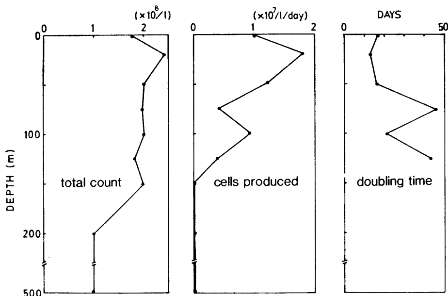
Fig. 4. Vertical profile of bacterial number, production rate, and doubling time at Stn. 5B.
