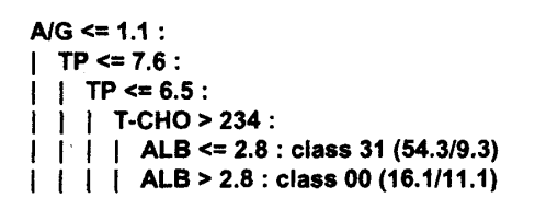
図10 決定木の例 Fig.10 Example of decision tree.
